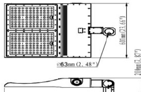
Slipfitter Mounting 450W/600W
