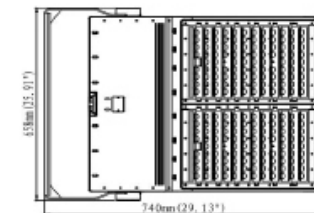
Straight Arm Mounting 450W 600W
